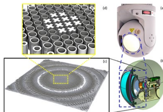
Above: (a) The Air Force fighter jet gimbal. (b) Schematic of the internal structure of the optical imaging assembly where the metalens is being inserted. (c) An image of the metalens designed by MIRaGE for the gimbal. (d) A zoom in image of the metalens core showing the different metamaterial unit cells.
